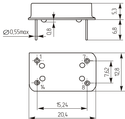
Full size (DIP14)
