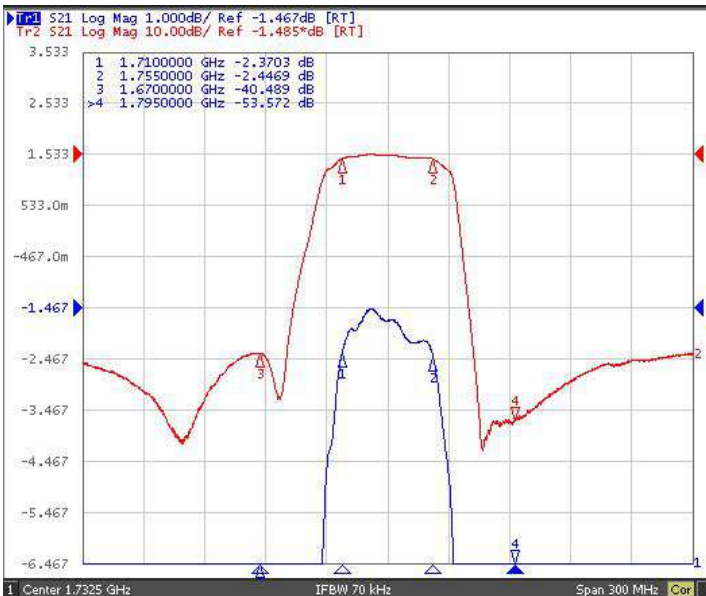
Frequency Response
