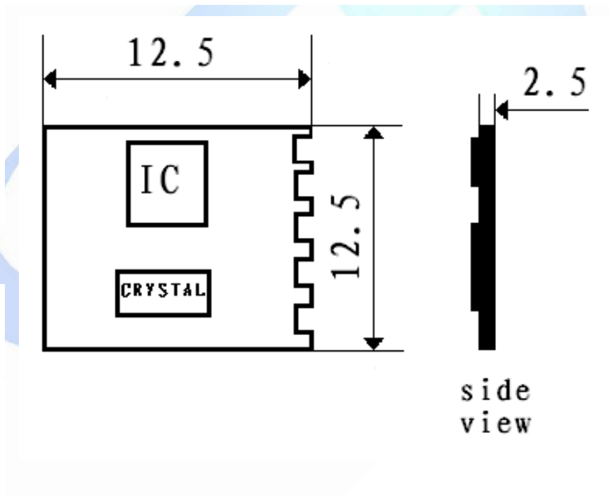
Figure2 CY89-V1.1 Dimension
