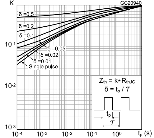
Figure 2. Thermal impedance
