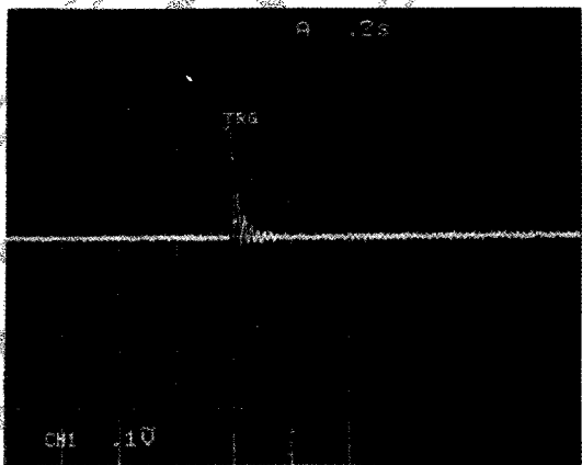
Locus when OFF Standby SW OFF V_{CC} = 13.2V R_L = 4\Omega R_g = 0
