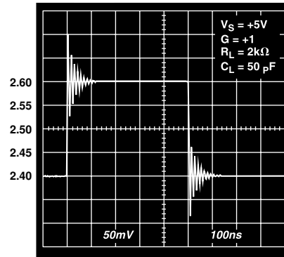
Figure 38. AD8051/AD8052 200 mV Step Response: C_L = 50pF
