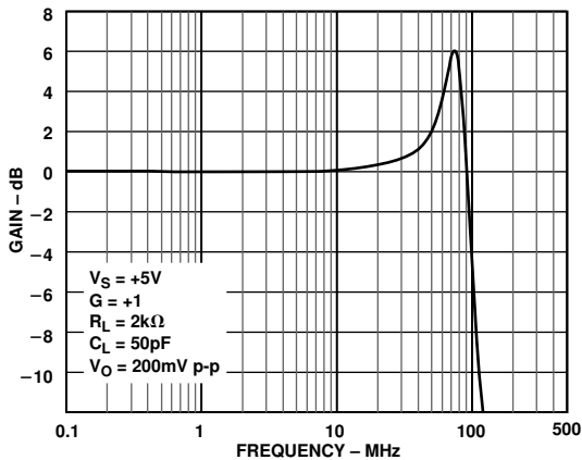
Figure 37. AD8051/AD8052 Closed-Loop Frequency Response: C_L = 50pF
