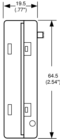
END VIEW
