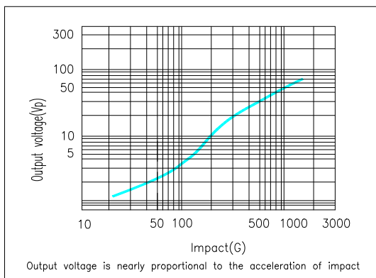
Output Voltage vs. Impact Response
