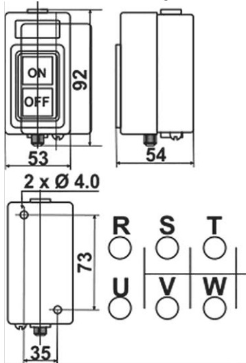
Outline Drawing
