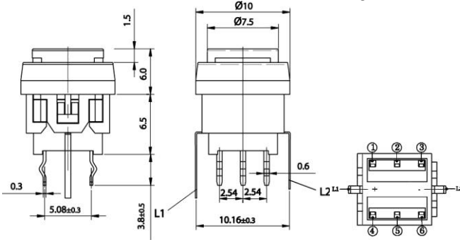
Outline Drawing
