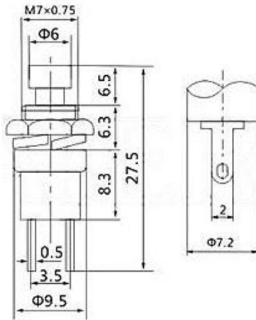
Outline Drawing
