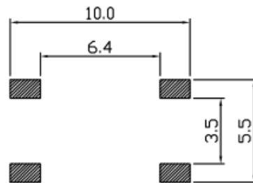
P. C. B LAYOUT
