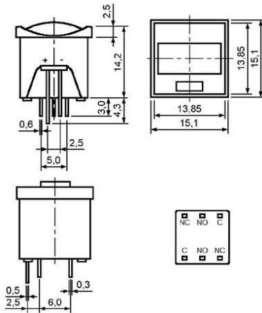
Outline Drawing
