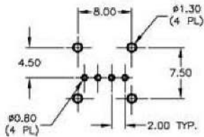
Mounting
