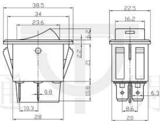
Outline Drawing
