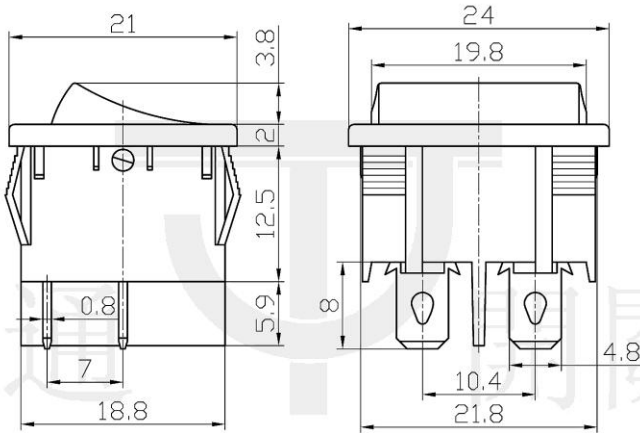
Outline Drawing
