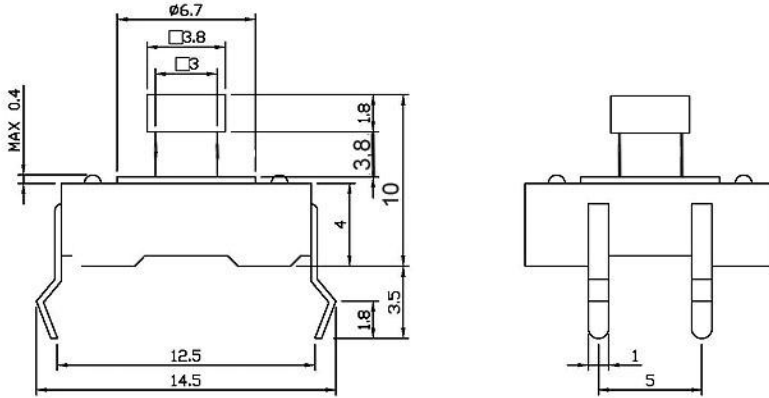
Outline Drawing
