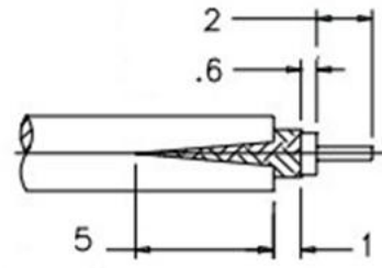
RECOMMENDED CABLE STRIPPING DIM'S
